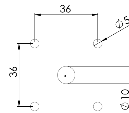
Bohrbild /Hole pattern
