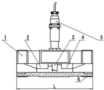
DN15~40 Sensor Structure & Installation Diagram
