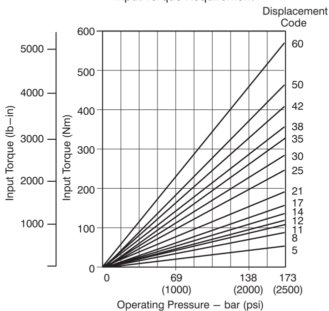
Input Torque Requirement
