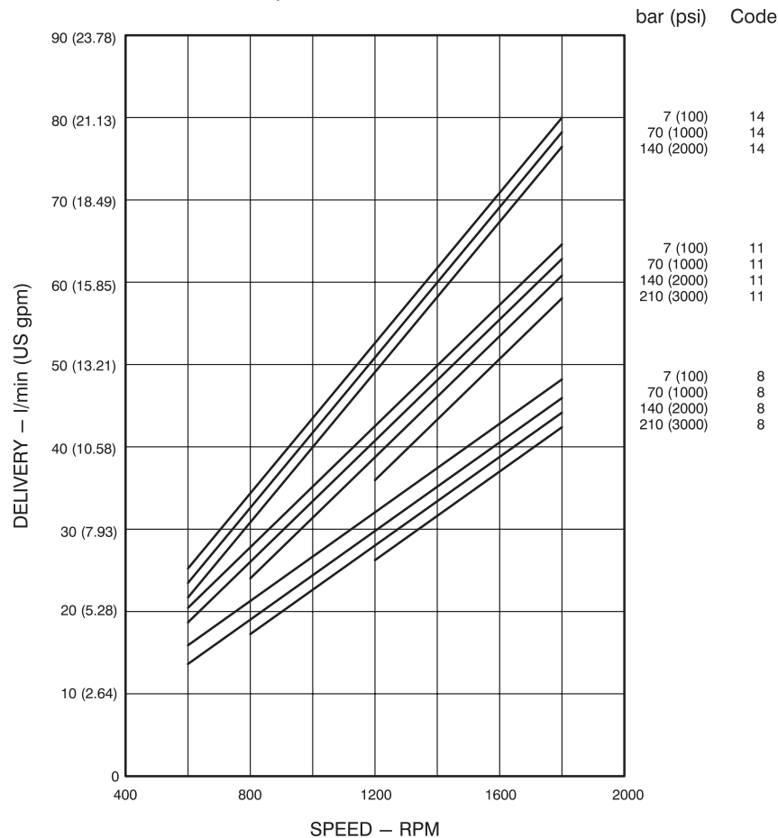
Codes 8, 11, and 14 Displacement
