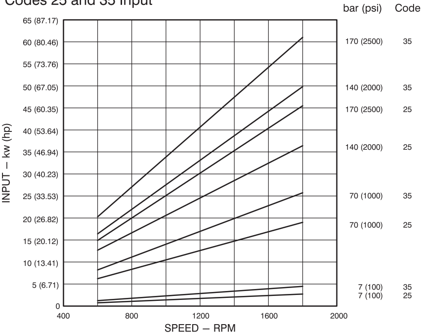
Codes 25 and 35 Input
