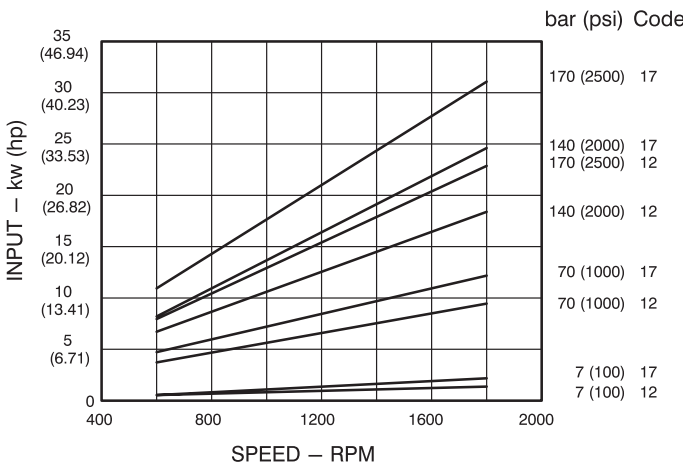
Codes 12 and 17 Input
