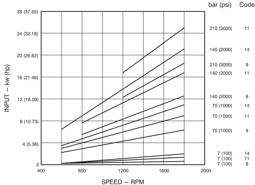
Codes 8, 11, and 14 Input
