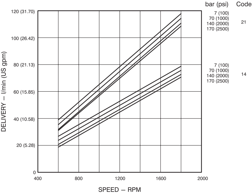
Codes 14 and 21 Displacement
