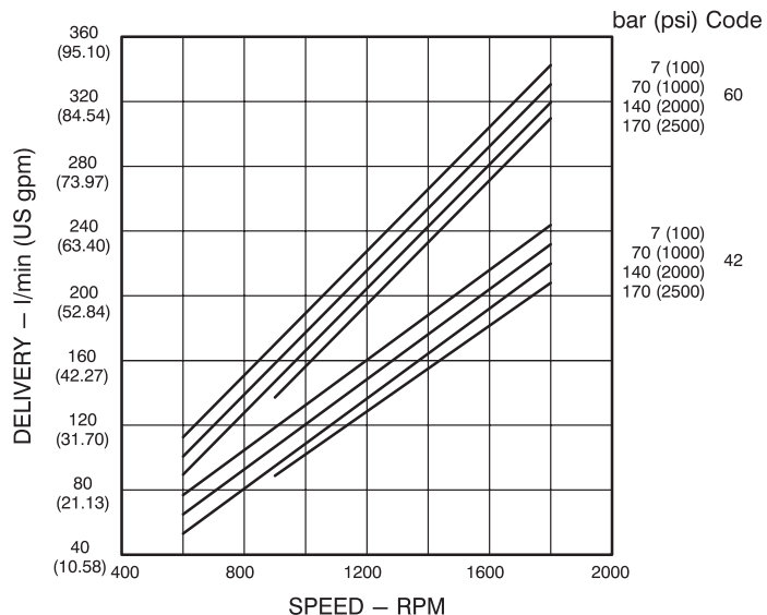
Codes 42 and 60 Displacement
