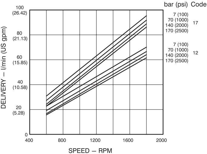
Codes 12 and 17 Input
