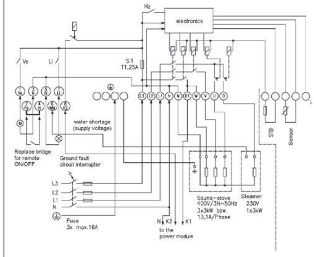
Circuit diagram, Hygrotherm VU
