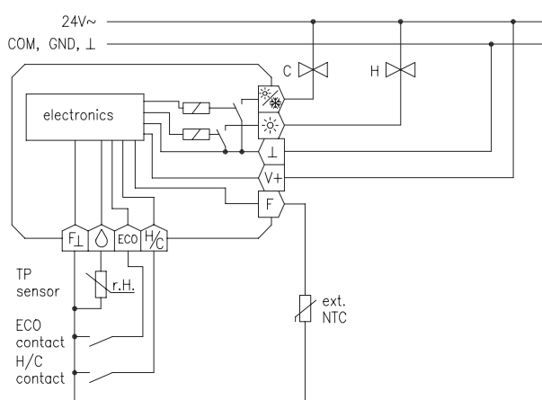
Circuit diagram KTRRU-052.24x in 4-pipe system
